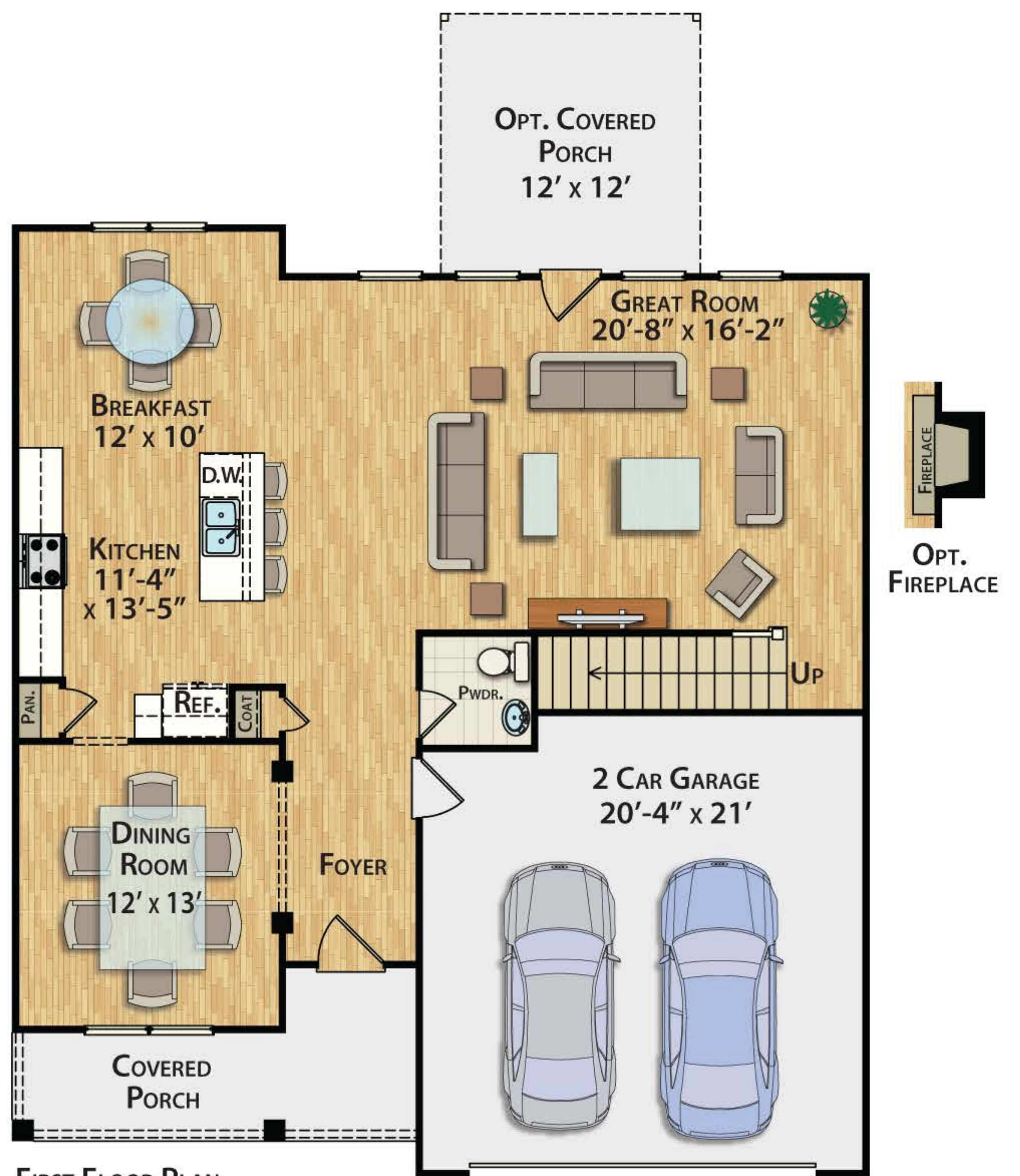
FIRST FLOOR PLAN JASPER
